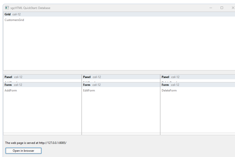
Figure 4.12. The form in Delphi: the boxes are the sgHTML grid and three panels, each holding a form. The label and button below them are plain VCL controls that do not appear on the web page.
