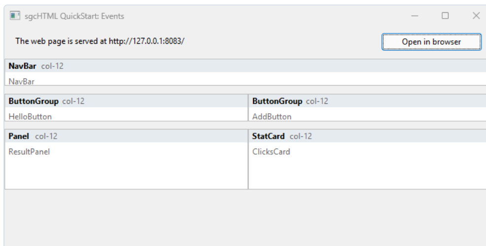
Figure 4.6. The form in Delphi: the boxes are the sgHTML components, the label and button above them are plain VCL controls that do not appear on the web page.
