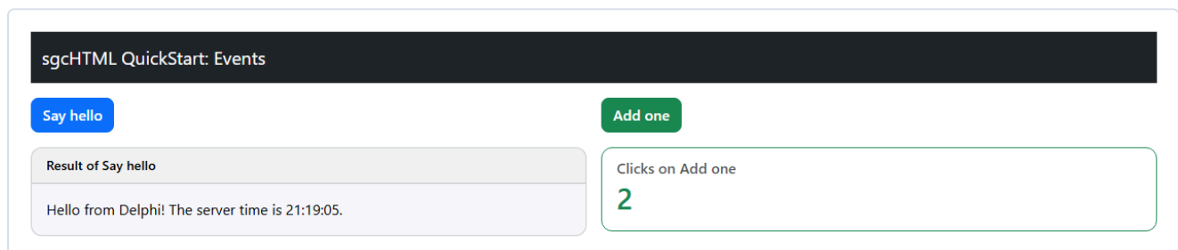
Figure 4.7. After one click on Say hello and two on Add one. Only the panel and the card changed.
