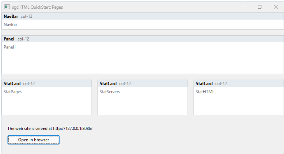
Figure 4.15. The main form in Delphi, which becomes the Home page. The NavBar box at the top is the navigation frame, the other boxes are sgHTML components, and the label and button below them are plain VCL controls that do not appear on the web page.
