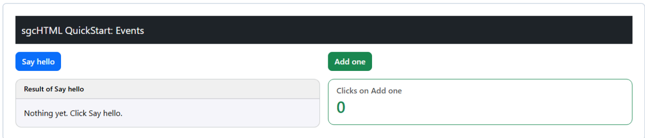
Figure 4.5. The Events page when it opens. The panel says Nothing yet and the counter shows 0.
